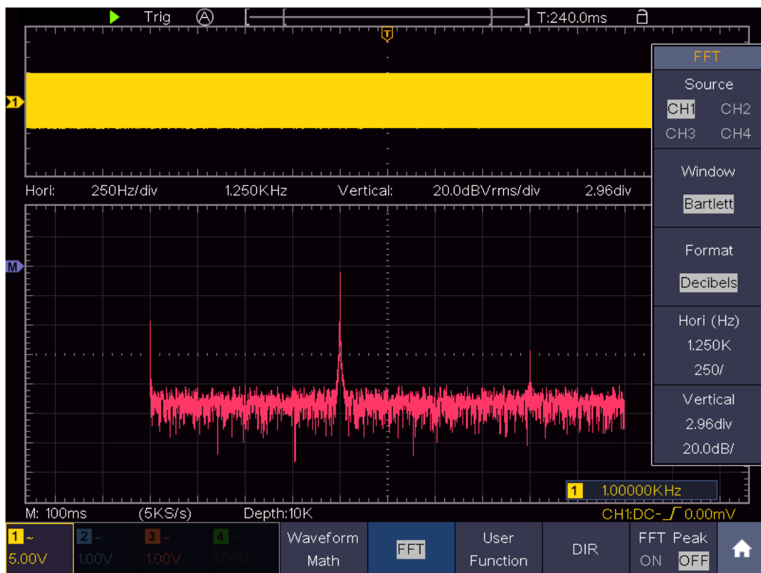
Figure 4-6 Bartlett window
