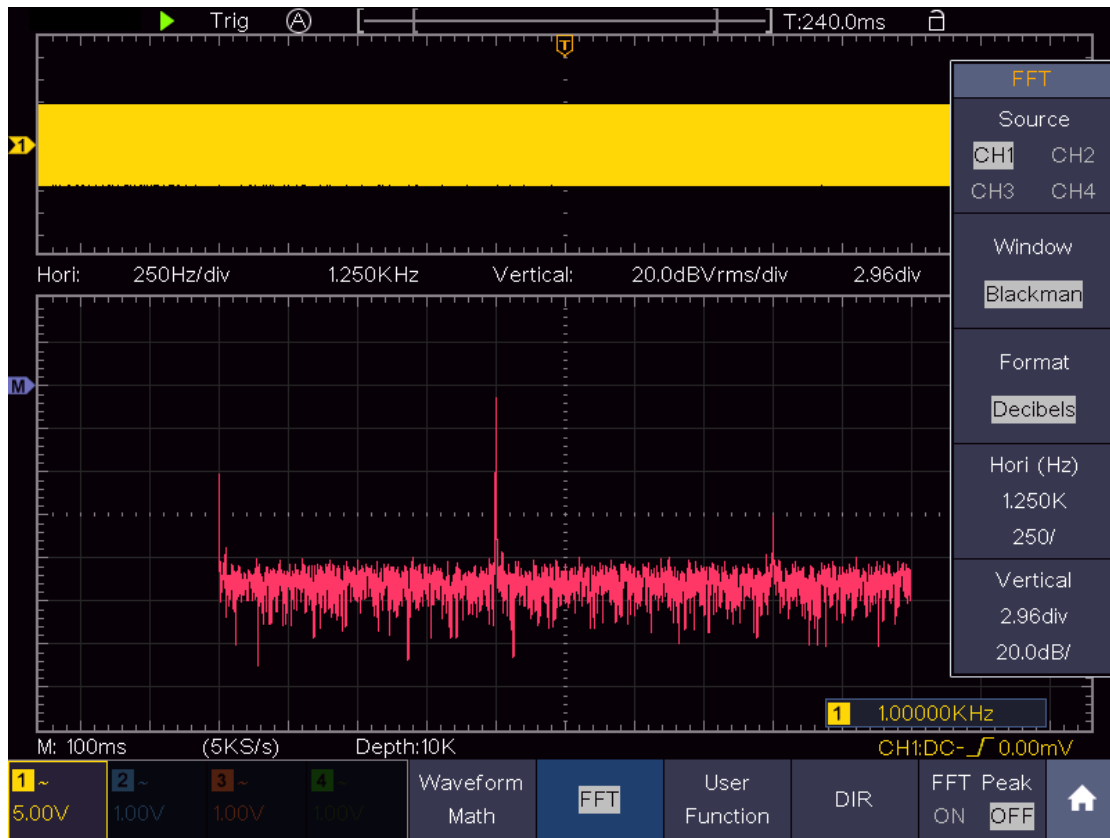
Figure 4-3 Blackman window
