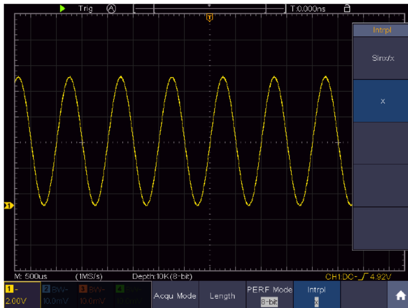
Figure 4-11 Linear interpolation
