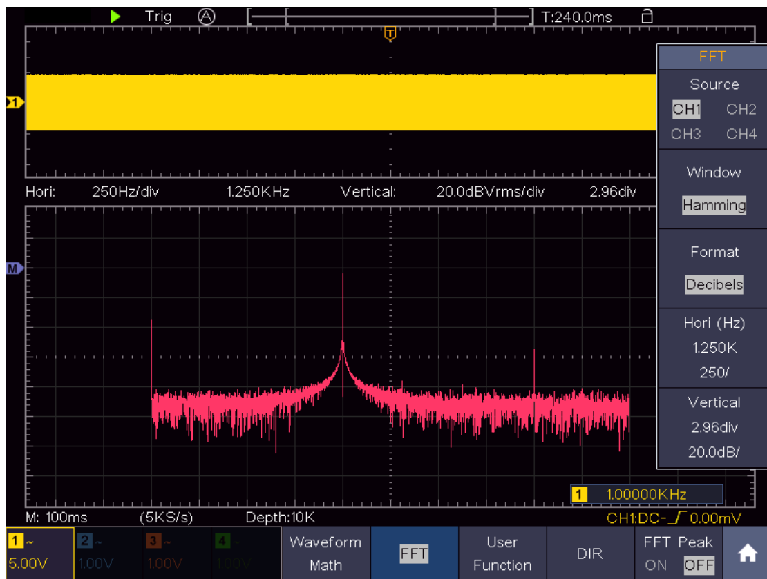
Figure 4-1 Hamming window
