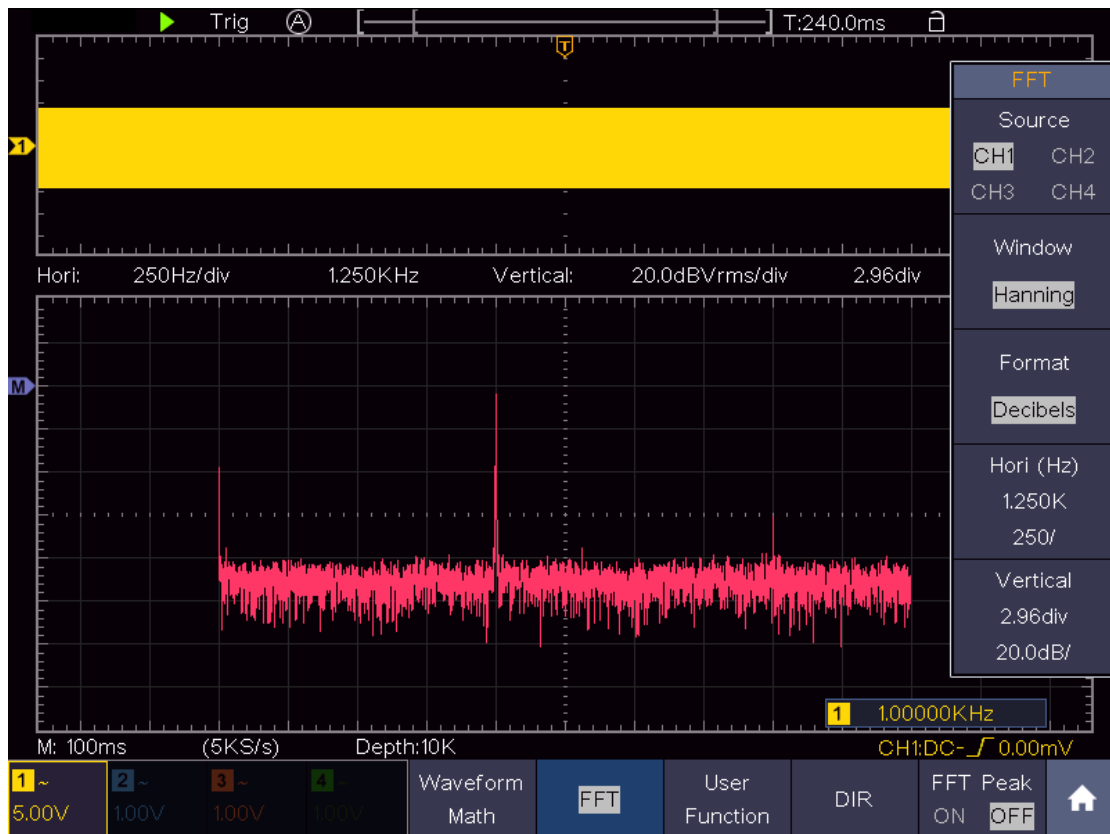
Figure 4-4 Hanning window
