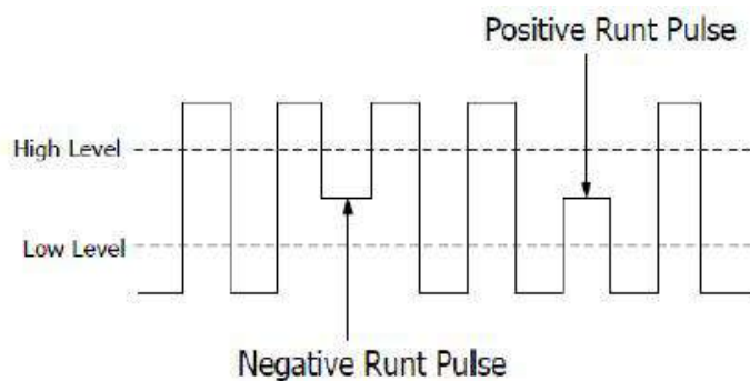
Runt Trigger
