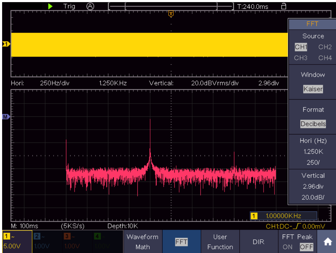
Figure 4-5 Kaiser window
