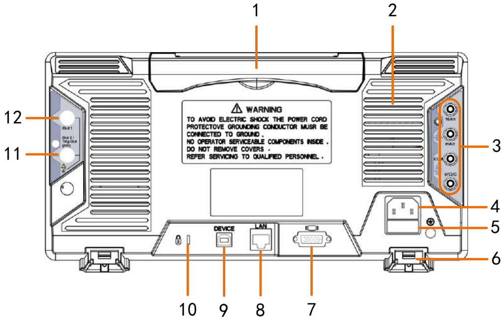
Figure 3-2 Rear Panel
